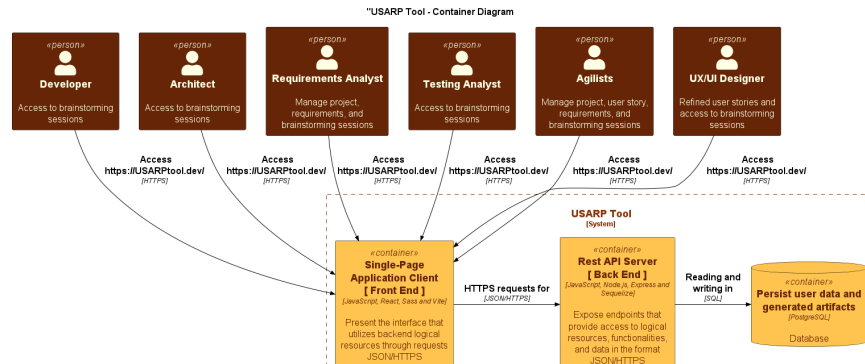
Fig. 2. Container diagram of the USARP Tool architecture using the C4 model.
