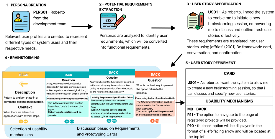
Fig. 1. The process updated to apply the USARP method.
