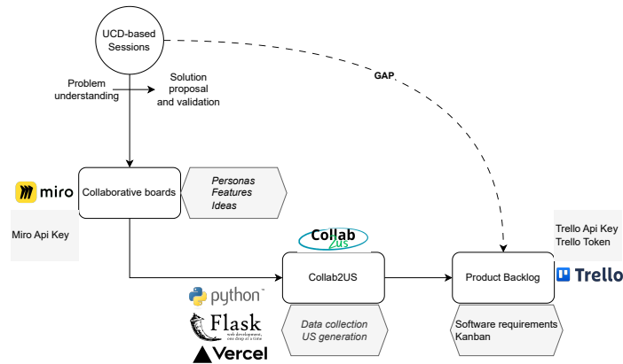
Fig. 2. Collab2US application scenario
